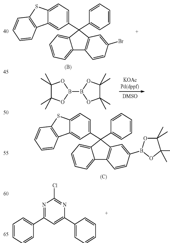
[Reaction Scheme 2]
