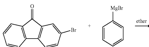
[Reaction Scheme 1]
