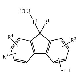
[Chemical Formula 1]
