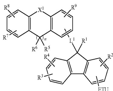
[Chemical Formula 3]
